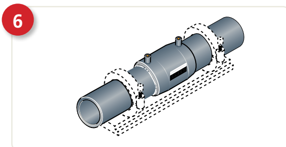
Align and clamp pipe
