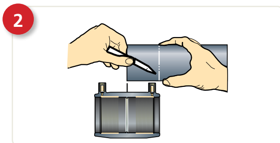
Mark stab depth on pipe
